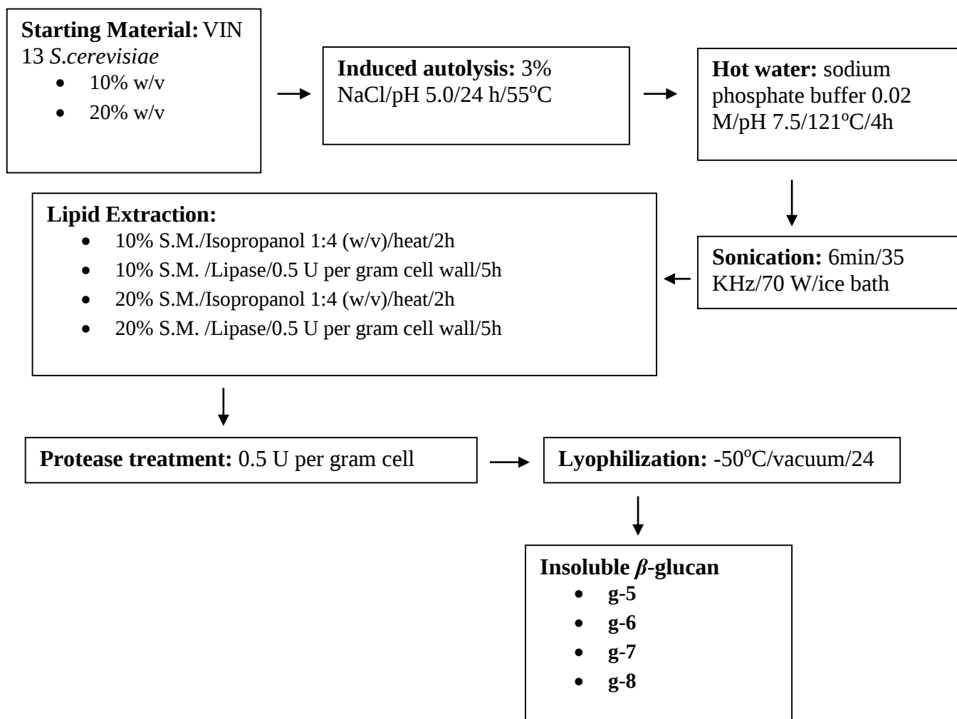
Fig. 2. Schematic diagram showing the process for the extraction of (1,3)(1,6)-β-D-glucan with extraction Method 2
